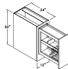
HUTCH BASE MEDIA - HBMED
