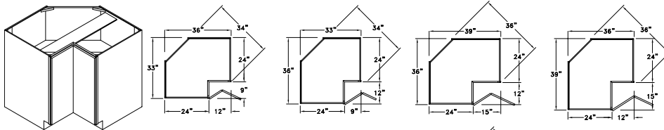
ASYMMETRICAL CORNER BASE - CBA
