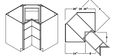
3 DRAWER CORNER BASE - CB3D
