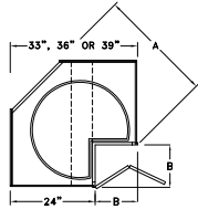
CORNER BASE LAZY SUSAN - CBL
