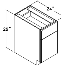
KITCHEN DESK BASE CABINET - KDBC
