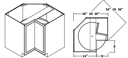
CORNER BASE WIRE LAZY SUSAN - CBWLS
