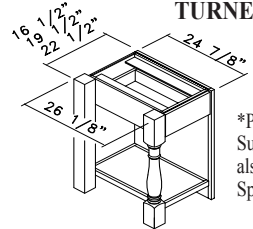
ISLAND SPICE DISPLAY - ISDB ISLAND PLATE DISPLAY - IPDB
