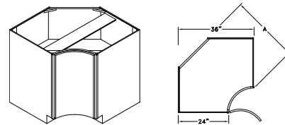
RADIUS BASE CORNER - RBC
