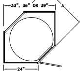
DIAGONAL BASE LAZY SUSAN - DBLS
