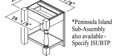
ISLAND SUB-ASSEMBLY W/ TURNED POSTS - ISUBT
