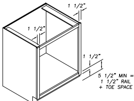
RANGE BASE - RB
