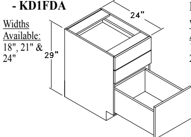
KITCHEN DESK FILE DRAWER STYLE A - KD1FDA
