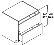
BASE PROFESSIONAL RANGETOP WITH DRAWERS - BPRTD
