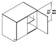
BASE PROFESSIONAL RANGETOP WITH DOORS - BPRTD
