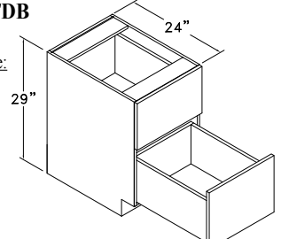
KITCHEN DESK FILE DRAWER STYLE B - KD1FDB
